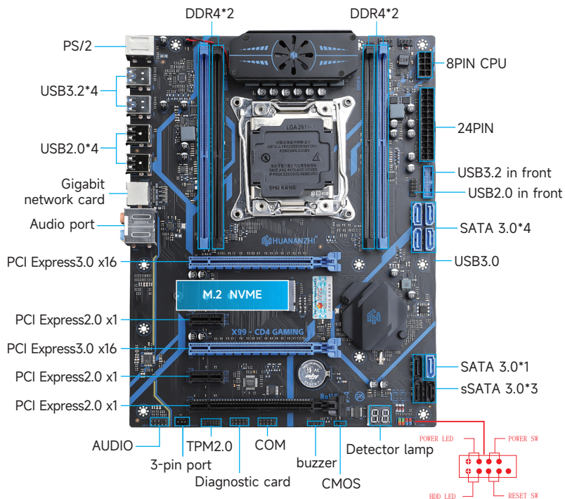
1-1 X99-CD4 GAMING Motherboard Illustration
