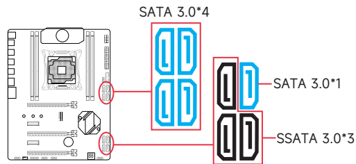
2 -10 SATA Interface
