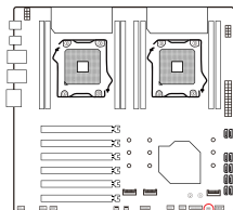
2-1 Clear CMOS Jumper CLR-CMOS
